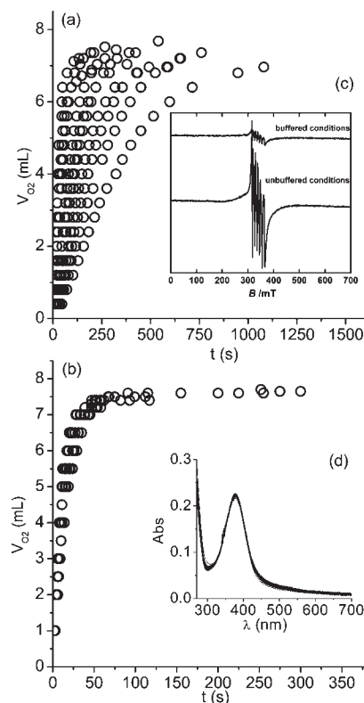
Figure 9. Time-dependence of \text{O}_2 evolution after successive additions of 63 \mu\text{L} of 10.05 \text{ M} \text{H}_2\text{O}_2 (175 equiv) to an (a) aqueous solution of 1 ( 1.2 \times 10^{-3} \text{ M} ) + 5 equiv NaOH; and (b) 1 in a buffer at pH 10.75. (c) EPR spectra taken at the end of \text{H}_2\text{O}_2 disproportionation in NaOH and a buffer; \nu = 9.5 \text{ GHz} , T = 100 \text{ K} , and microwave power = 0.5 \text{ mW} . (d) Electronic spectra registered after successive additions of \text{H}_2\text{O}_2 to the solution of 1 ( 1.1 \times 10^{-5} \text{ M} ) in a buffer at pH 10.75 and T = 298 \text{ K} .
