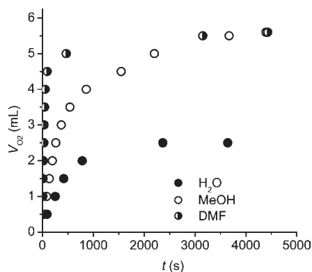
Figure 8. Time-dependence of \text{O}_2 evolution upon reaction of 1 with 150 equiv of \text{H}_2\text{O}_2 in different solvents. [\mathbf{1}] = 1 \times 10^{-3} \text{ M} ; T = 25^\circ \text{C} .
