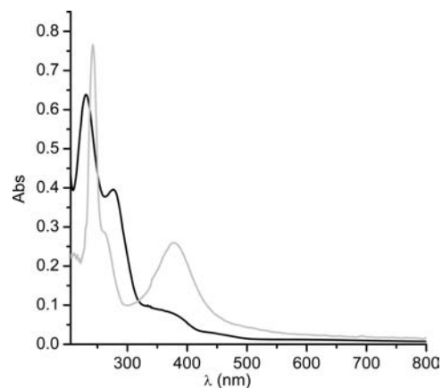
Figure 5. Electronic spectra of 1.3 \times 10^{-5} M 1 in H 2 O (black) and buffer of pH 10.75 (gray); l = 1 cm.
