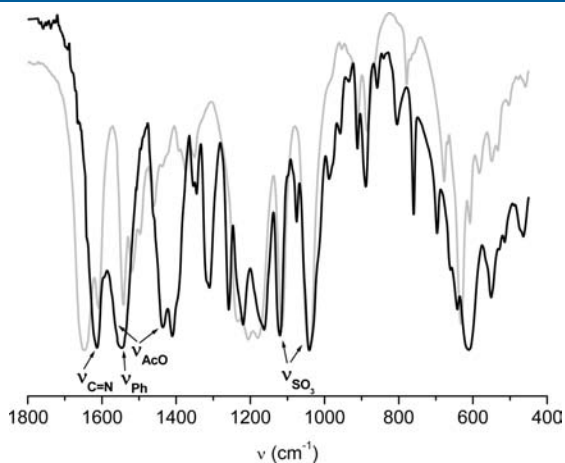
Figure 1. FT-IR spectra of complex 1 (black) and \text{Na}_2[3\text{-Me-5-SO}_3\text{-salpentOH}] (gray).
